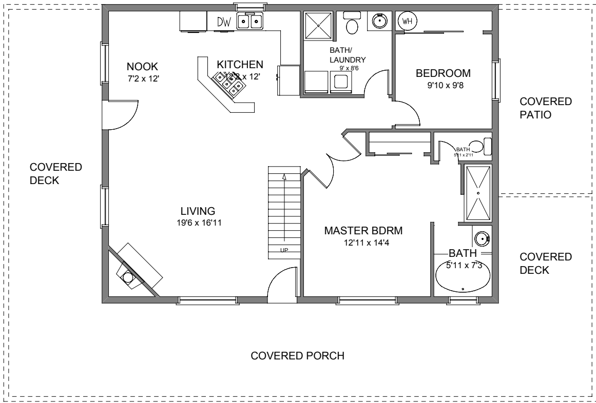
Bent Tree Ranch First Floor APPROXIMATE LIVING AREA 1226 sq ft
